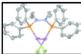
Fig. 1. Molecular structure drawn with displacement ellipsoids at the 50% probability level. Hydrogen atoms and solvent THF have been omitted for clarity.
